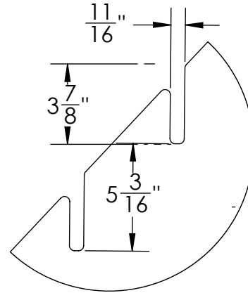
DETAIL B SCALE 2 : 13
