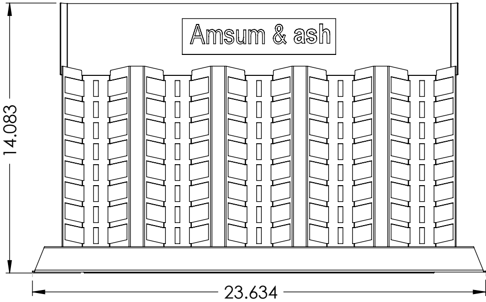
ALL SHEET-METAL STRUCTURE, POWDERCOATED CUSTOM COLOR
